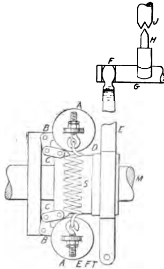
FIG. 365.—One type of Gas Engine Governor, which is an improved variation of the device used on the early Daimler motors. The parts are as follows: A and A, ball weights; B and B', bell cranks actuating the links, C and C', as the balls move outward resisting the tension of spring, S, and sliding sleeve, D, on the shaft, M. E is a lever arm attached to D, which moves the shaft, G, by contact at F, as shown, thus throwing the pick blade, H, out of contact with the end, J, of the exhaust valve rod.
